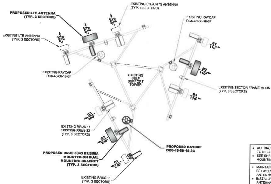
FINAL ANTENNA LAYOUT
