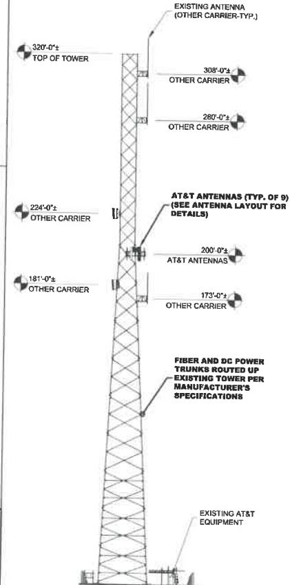
TOWER ELEVATION
